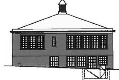
2 NORTH ELEVATION EXIST. GROUP
