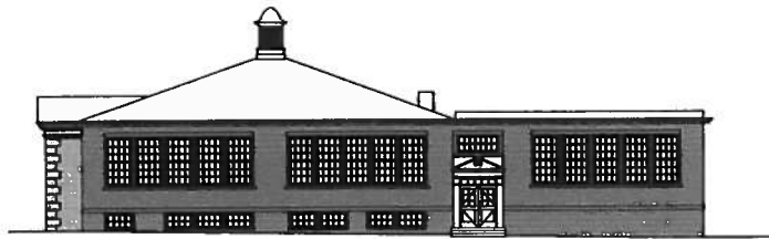
3 EAST ELEVATION EXIST. GROUP
